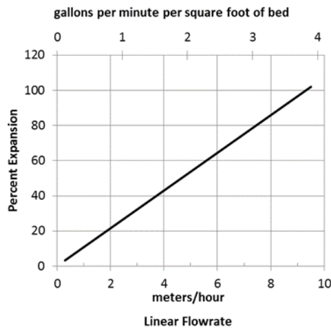
Figure 1: Backwash Expansion
