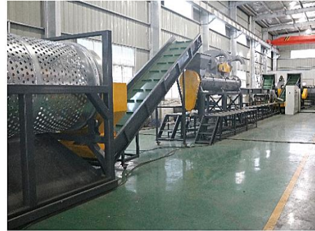
MT-1000 PET Washing Line in Yemen
